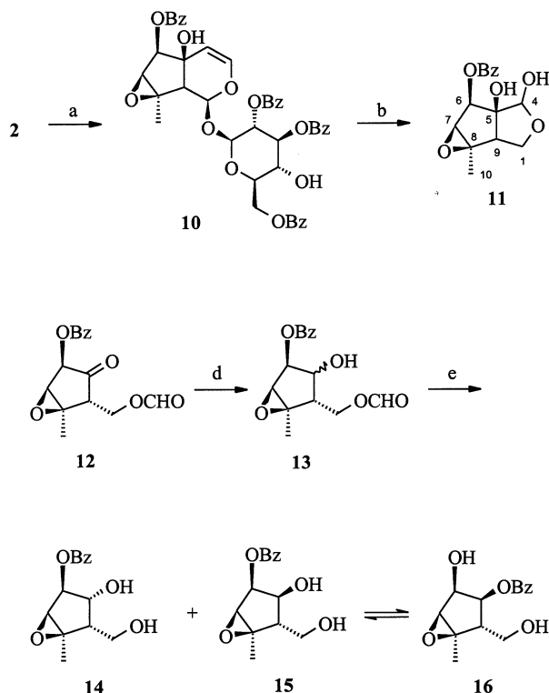
Scheme 2. Synthesis of the cyclopentanoid compound 14
