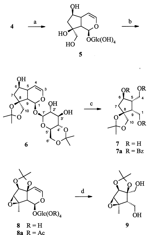
Scheme 1. Syntheses of cyclopentanoid compounds 7 and 9
